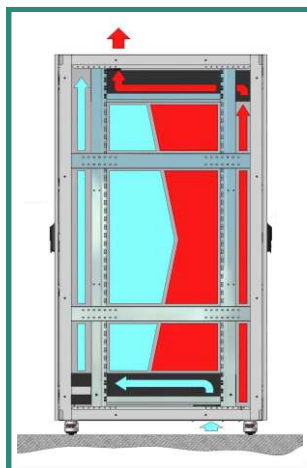
Efficient ventilation system with active noise reduction, bottom cold air intake and hot air exhaust at the top
