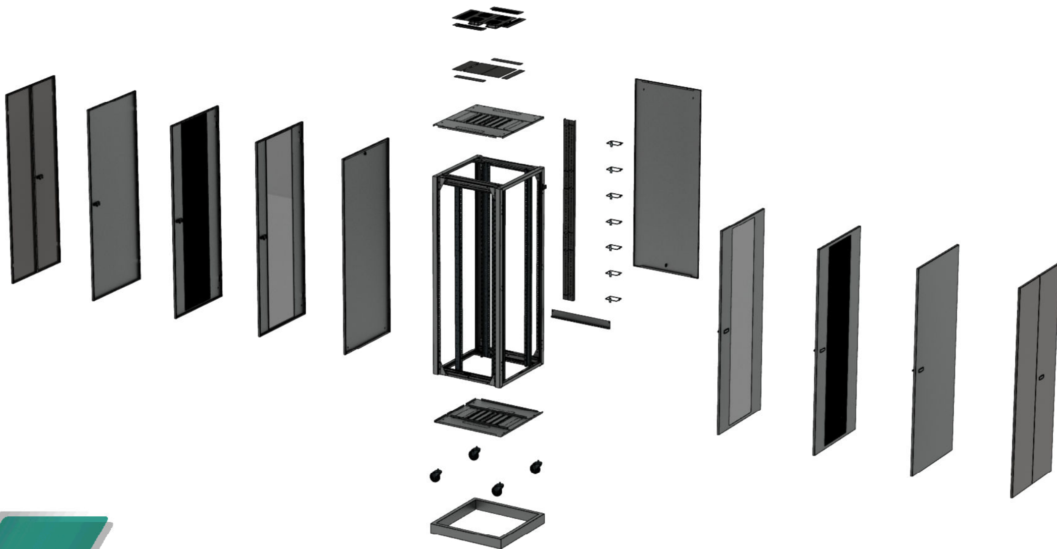
eCom 19" omara, širina 800mm
